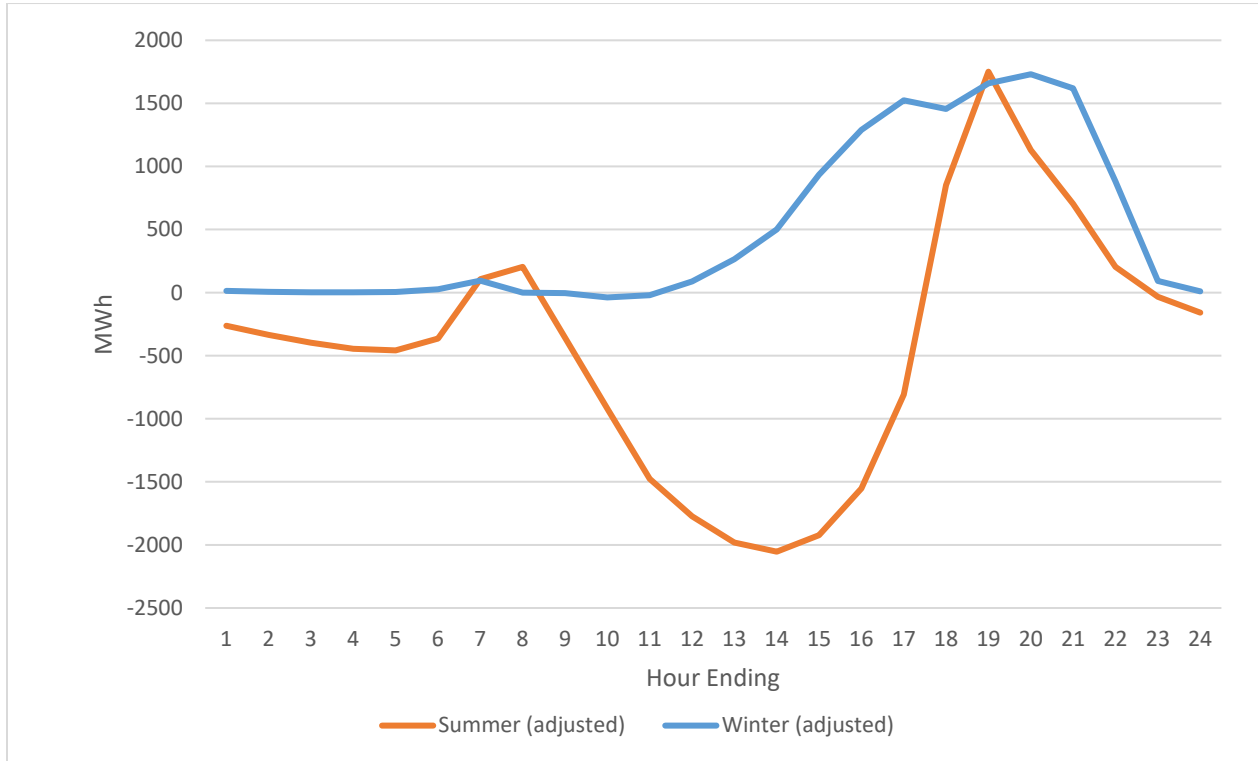
Figure 4. 2010-2020 interchange adjusted by CA heat rate analysis.
