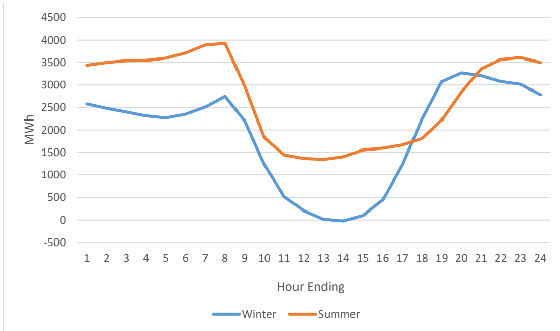
Figure 2. Raw regional Interchange 2018-2020 - declining daytime exports and peaks in morning and evenings. Roughly follows California solar production.
